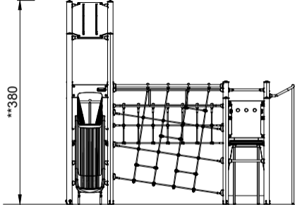
PCM410421 1:100
